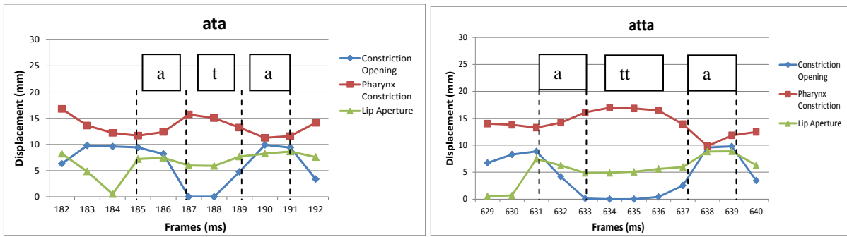
Figure 5: Trajectory of three articulatory parameters (constriction opening, pharynx constriction and lip aperture) of /ata/ (left) and /atta/ (right); speaker F.
